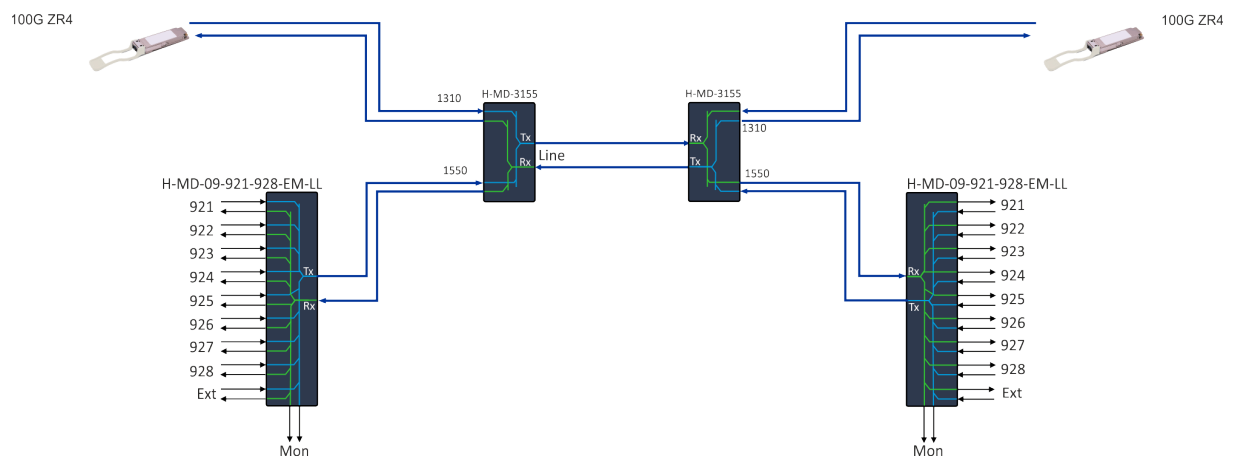
Figure 56: Mixed 1x 100G and DWDM configuration example
