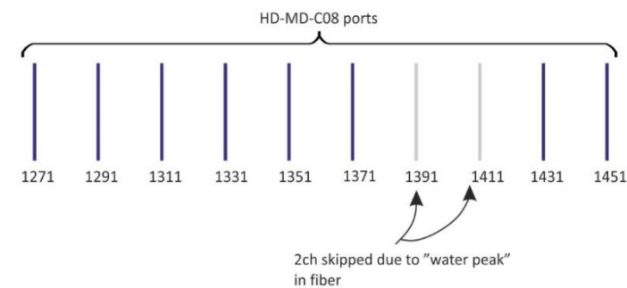
Figure 12: H-MD-C08 channels
