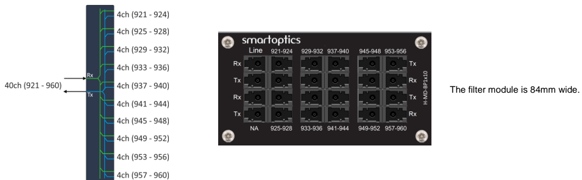
Figure 45: H-MD-BP1x10 icon and front plate
