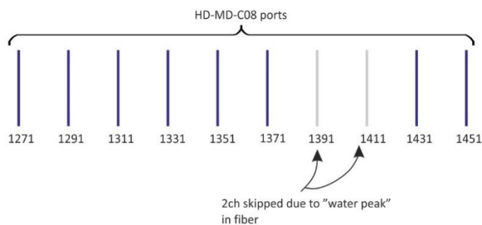
Figure 14: H-MD-C08L-LL channels
