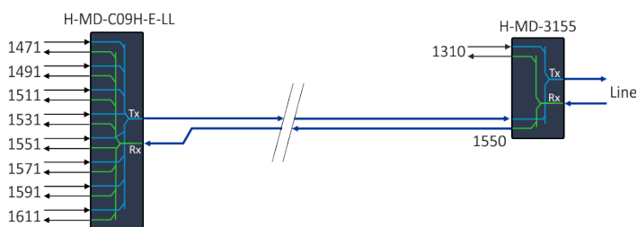
Figure 54: Mixed 1310nm legacy and CWDM configuration example
