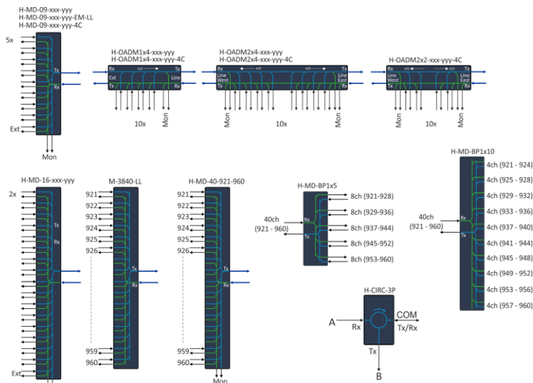
Figure 23: DWDM filters
