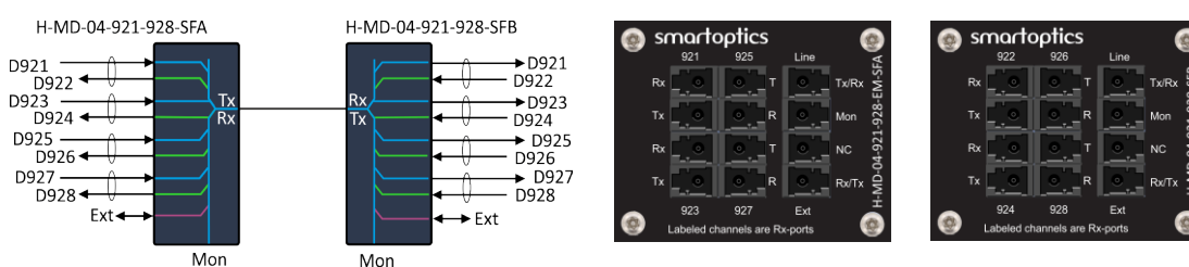
Figure 49: H-MD-04-921-928-SFx icons and front plates
