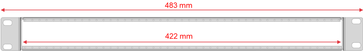
Figure 57: H-CHASSI-1RU
