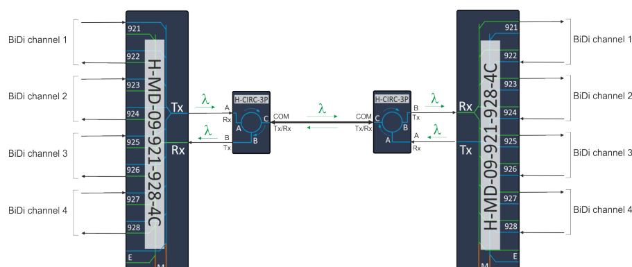
Figure 48: Single-fiber configuration example
