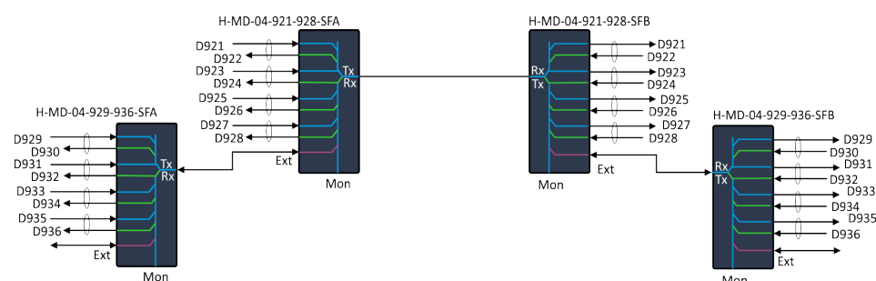
Figure 51: 8ch configuration
