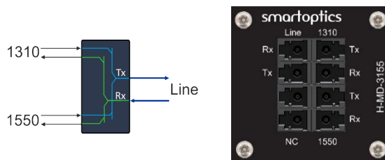
Figure 53: H-MD-3155 icon and front plate
