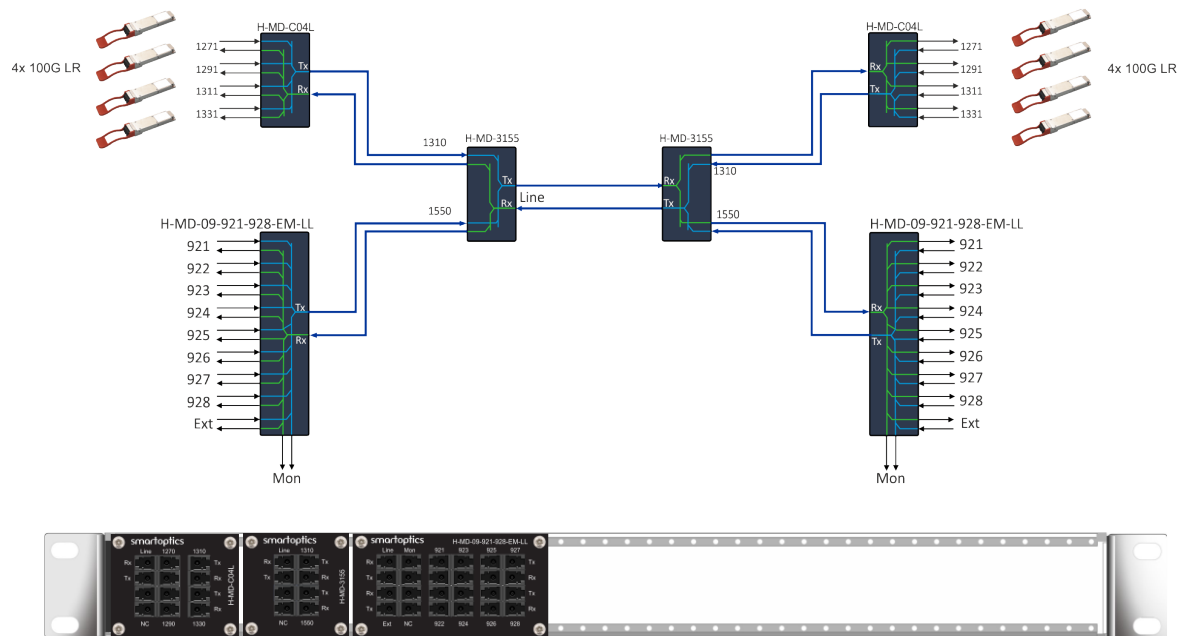
Figure 55: Mixed 4x 100G and DWDM configuration example
