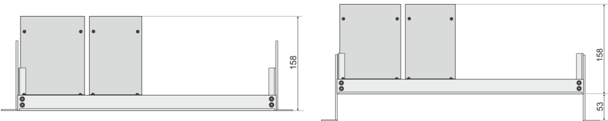
Figure 59: Mounting bracket positions
